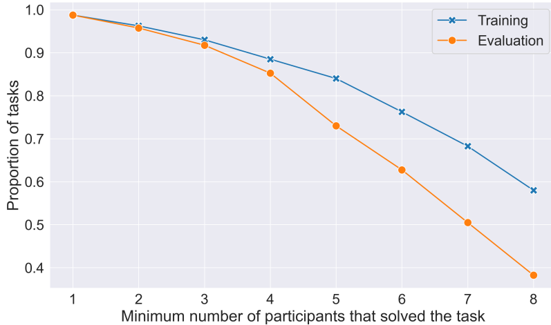
Figure 5: Minimum number of correct submissions across tasks. In this figure, we report the proportion of tasks where a minimum of N (x-axis) participants submitted a correct solution in three attempts or less. Note that higher values of N are biased negatively since posterior inference on a binomial outcome with small sample size is skewed.
