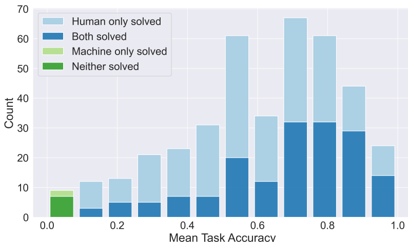
Figure 7: Human-machine performance comparison. In this figure, we compare human (2-shot) performance with GPT-4o-NS. We show the proportion of tasks solved by humans or machine only, both and neither for varying levels of human performance. We find 225 tasks that were only solved by humans, 7 tasks solved by neither and 2 tasks solved only by GPT-4o-NS.
