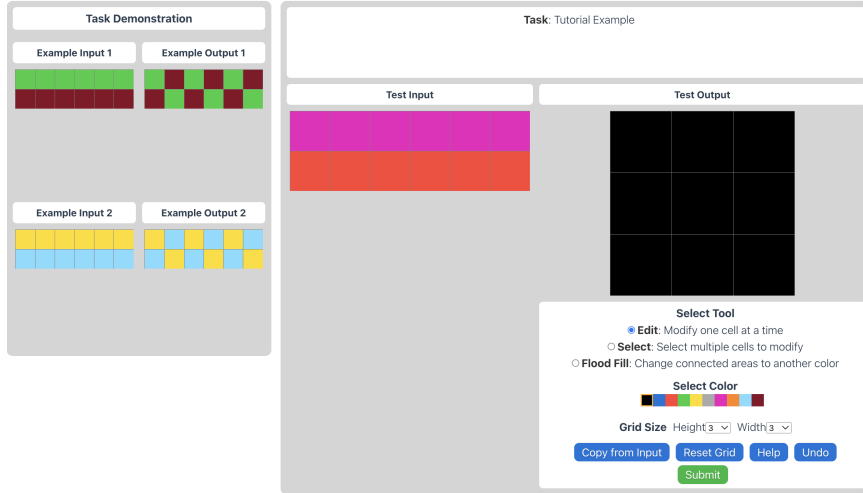
Figure 2: ARC Experiment Interface. Participants were given instructions about the different controls and layout of the interface followed by a tutorial task. Shown here is the evaluation tutorial task e9afcf9a.json .
